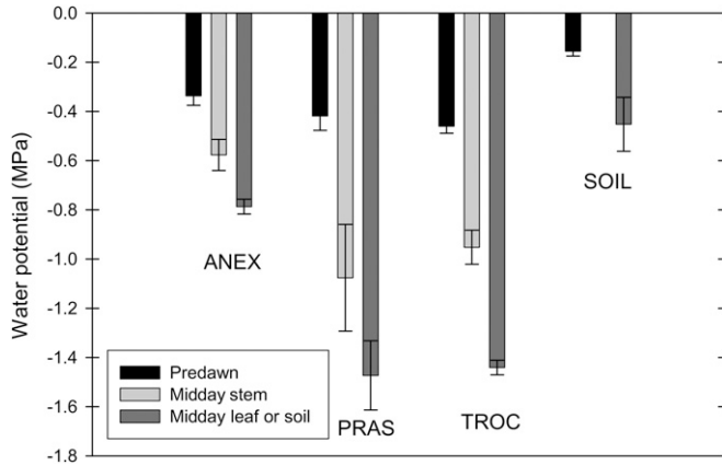
Fig. 2. Predawn leaf, midday leaf, and midday stem water potentials in Anacardium excelsum (ANEX), Prionostemma aspera (PRAS), and Trichostigma octandrum (TROC) and estimated predawn and midday soil (SOIL) water potentials.
