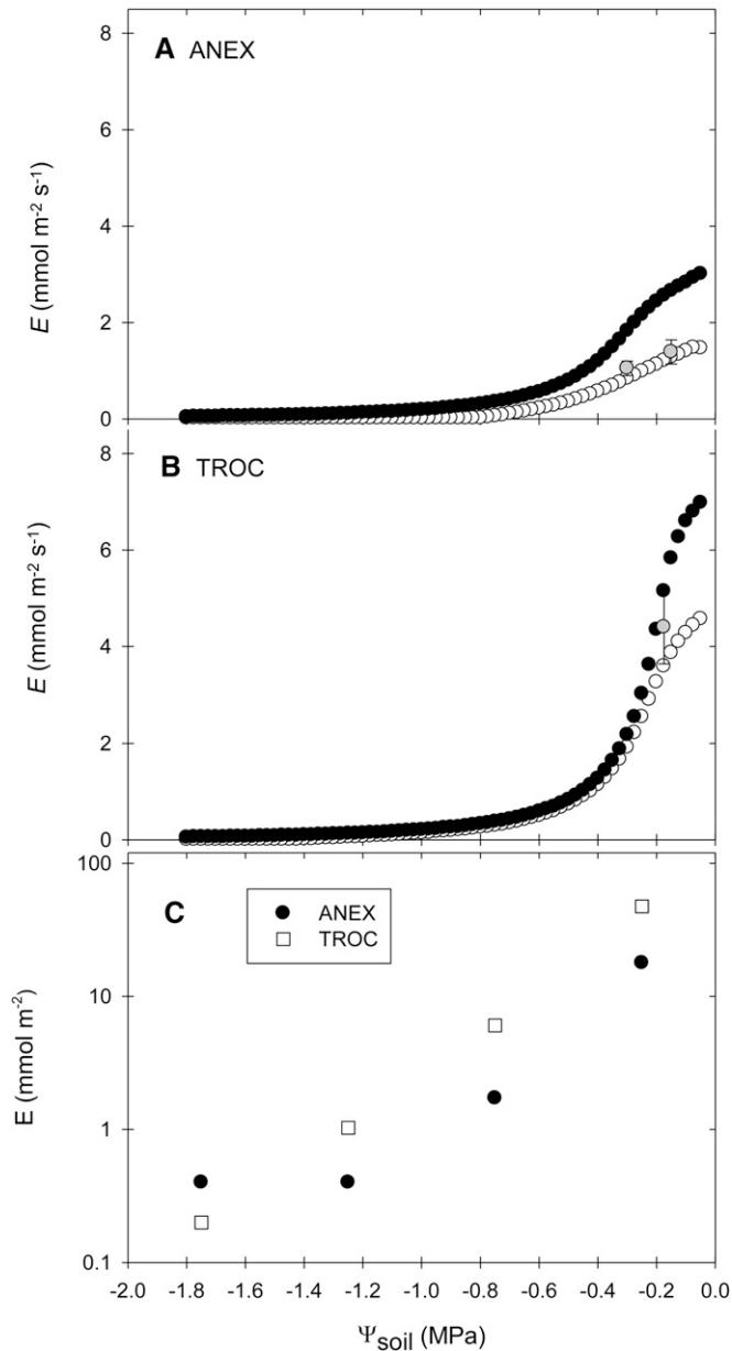
Fig. 4. Modeled and measured transpiration vs. soil water potential for the tree (A) Anacardium excelsum (ANEX) and the liana (B) Trichostigma octandrum (TROC). Closed circles represent the upper value for transpiration that would result in critical hydraulic failure ( E_{crit} ). Open circles represent predicted transpiration at a given soil water potential, and gray circles indicate measured values. Panel C is an estimate of plant water use integrated across ranges of soil water potentials (0 to -0.5 MPa, -0.5 to -1 , -1 to -1.5 , and -1.5 to -2.0 ). Closed circles represent ANEX, and open squares represent TROC.
